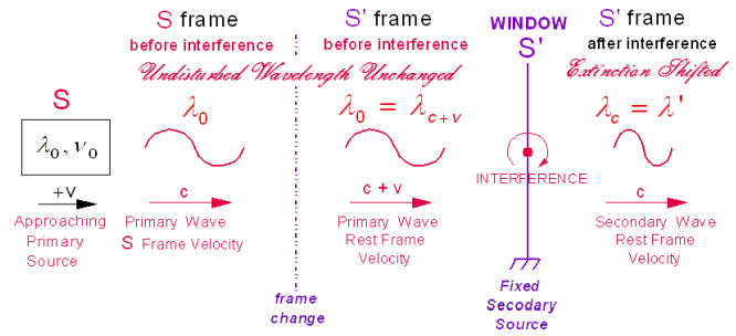
Fig. 2: A Reference Frame Independent Primary Wave is re-emitted as a Secondary Wave whose wavelength is consequently extinction shifted .
