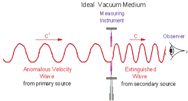
Fig. 1: An interfering observer attempts to measure a previously undisturbed primary wave emitted from a primary source of a different frame of reference other than that of the observer.
