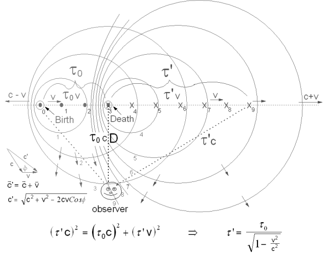
Fig. 3: A Transverse Relative Time Shift as opposed to Time Dilation assumed by Relativity .
