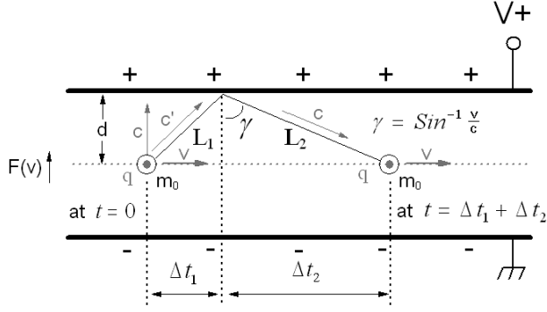
Fig. 4: An Effective Mass as opposed to Relativistic Mass as a function of velocity v relative to the frame of reference of the accelerating apparatus.
