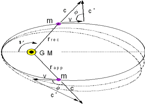
Fig. 5: A direct application of the Extinction Shift Principle calculates the perihelion rotation effect due a transit time effect for an exchange of gravitons between orbiting mass bodies according to Galilean transformations in Euclidean Space.
